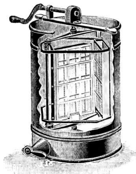
Extractor Cowan Rápido. British Beekeeper Guide Book, Ed. XX.
