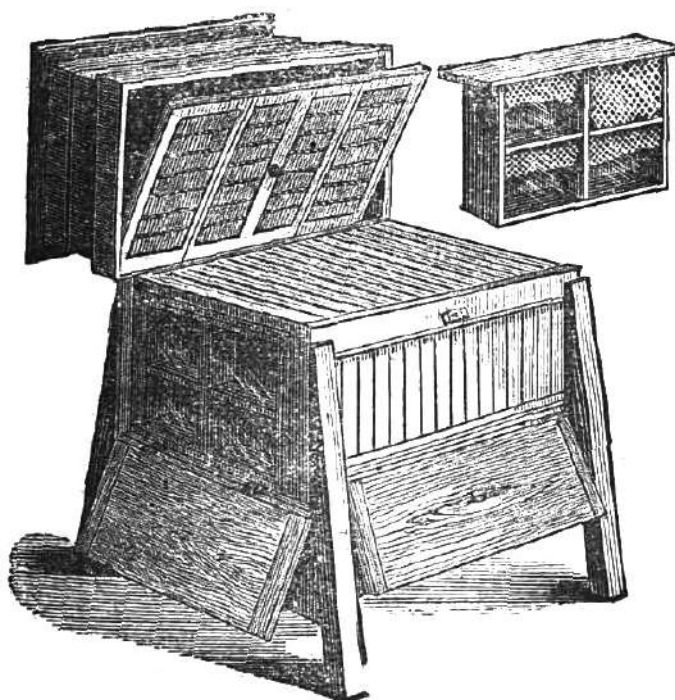
Fig. 23. Colmena colateral Kilburn.
